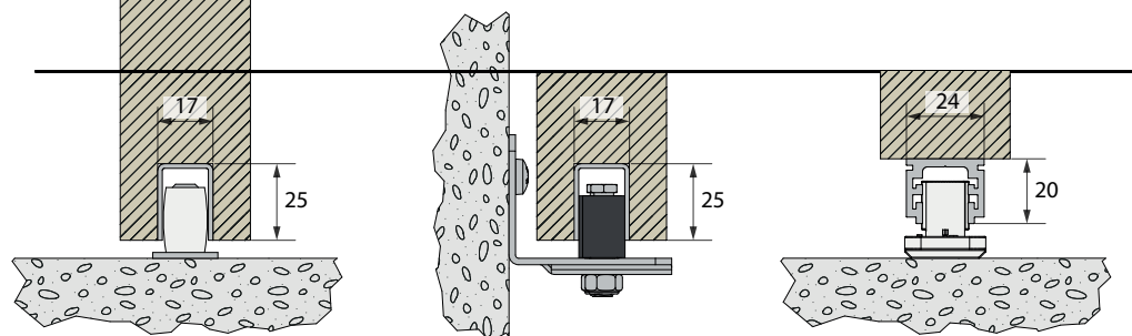
U-profile: 1109 Guide: 1102XA2
